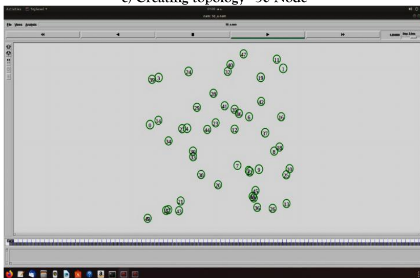
Figure 9: 50 Node topology
