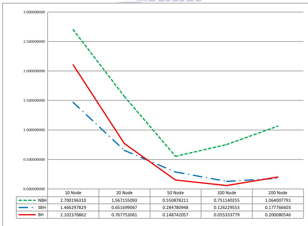
Figure 15: End To End Delay Chart
