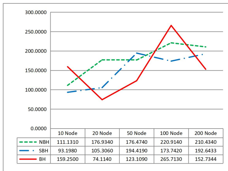
Figure 18: PDR Comparison in different time
