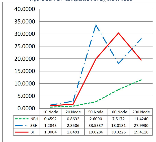
Figure 20: PDR Comparison in different node
