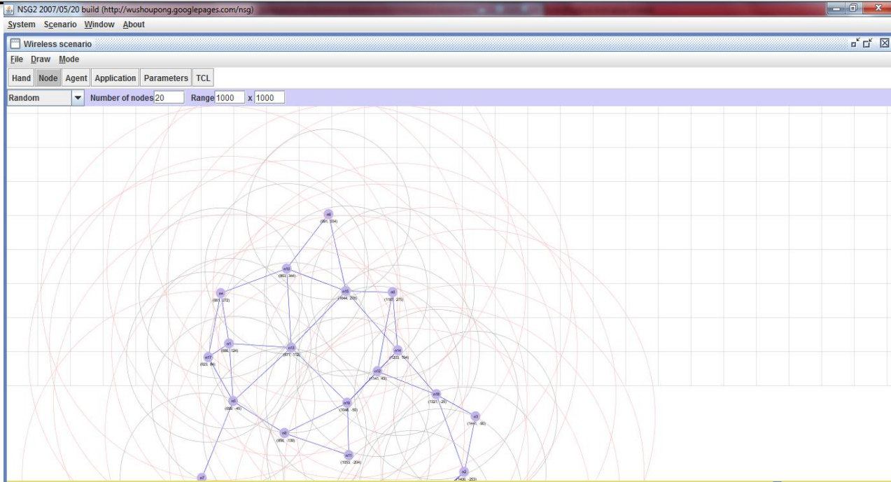
Figure 6: NS 2.35 Environment
