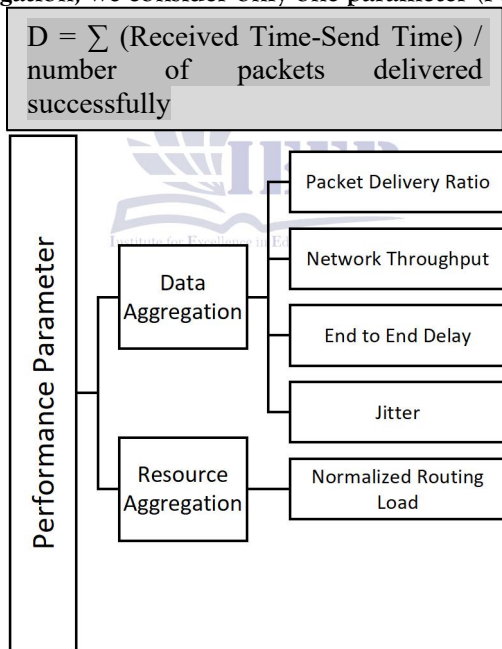
Figure 12: Performance Parameter
