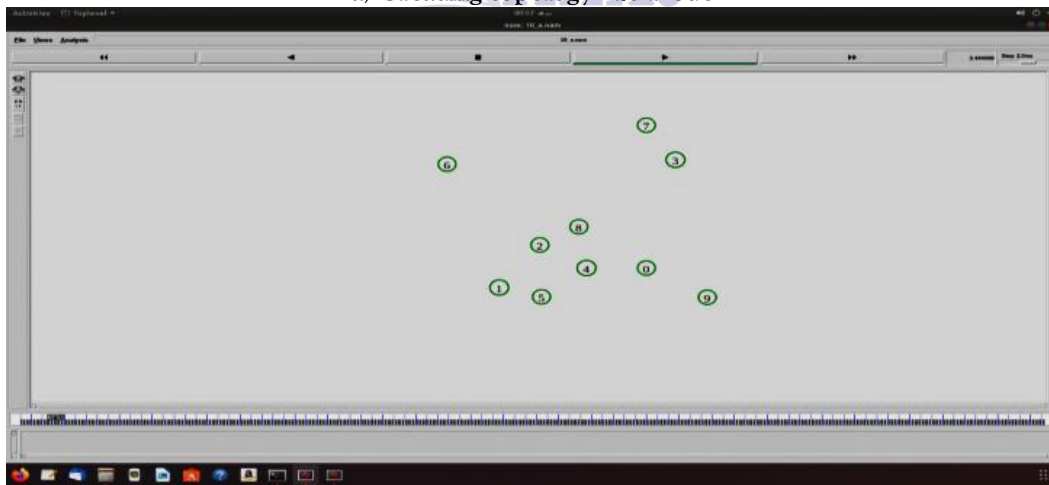
Figure 7: 10 Nodes
