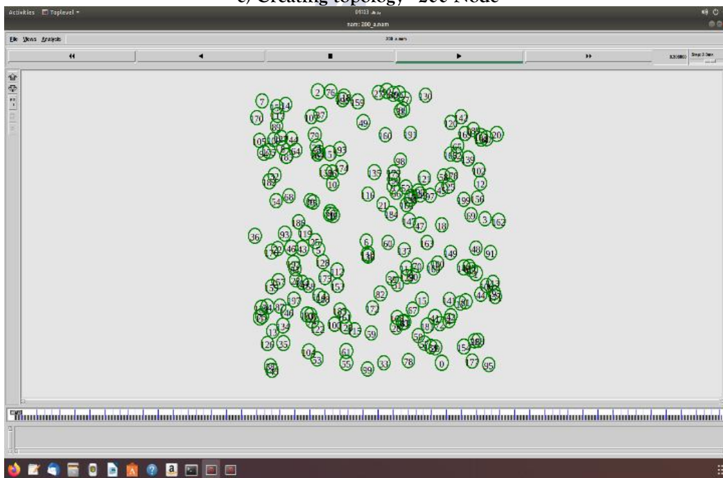
Figure 11: 200 Node Topology
