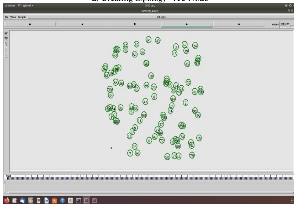
Figure 10: 100 Node Topology
