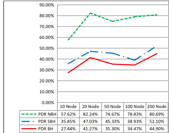
Figure 13: Packets Delivery Ratio Chart
