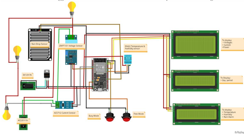
Fig12. Circuit Diagram
