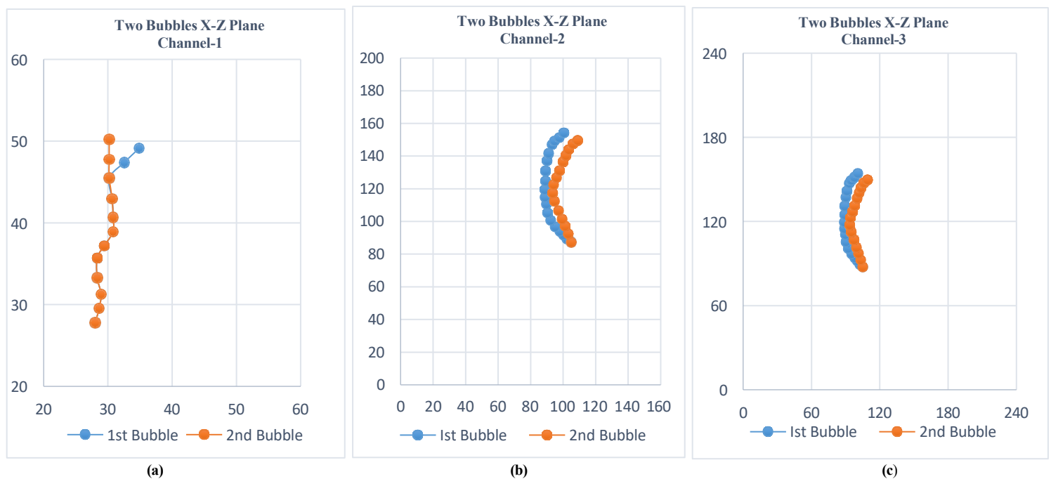
Figure 3.10(a-c): Graphical depiction of two bubble's rise in x-z plane.
