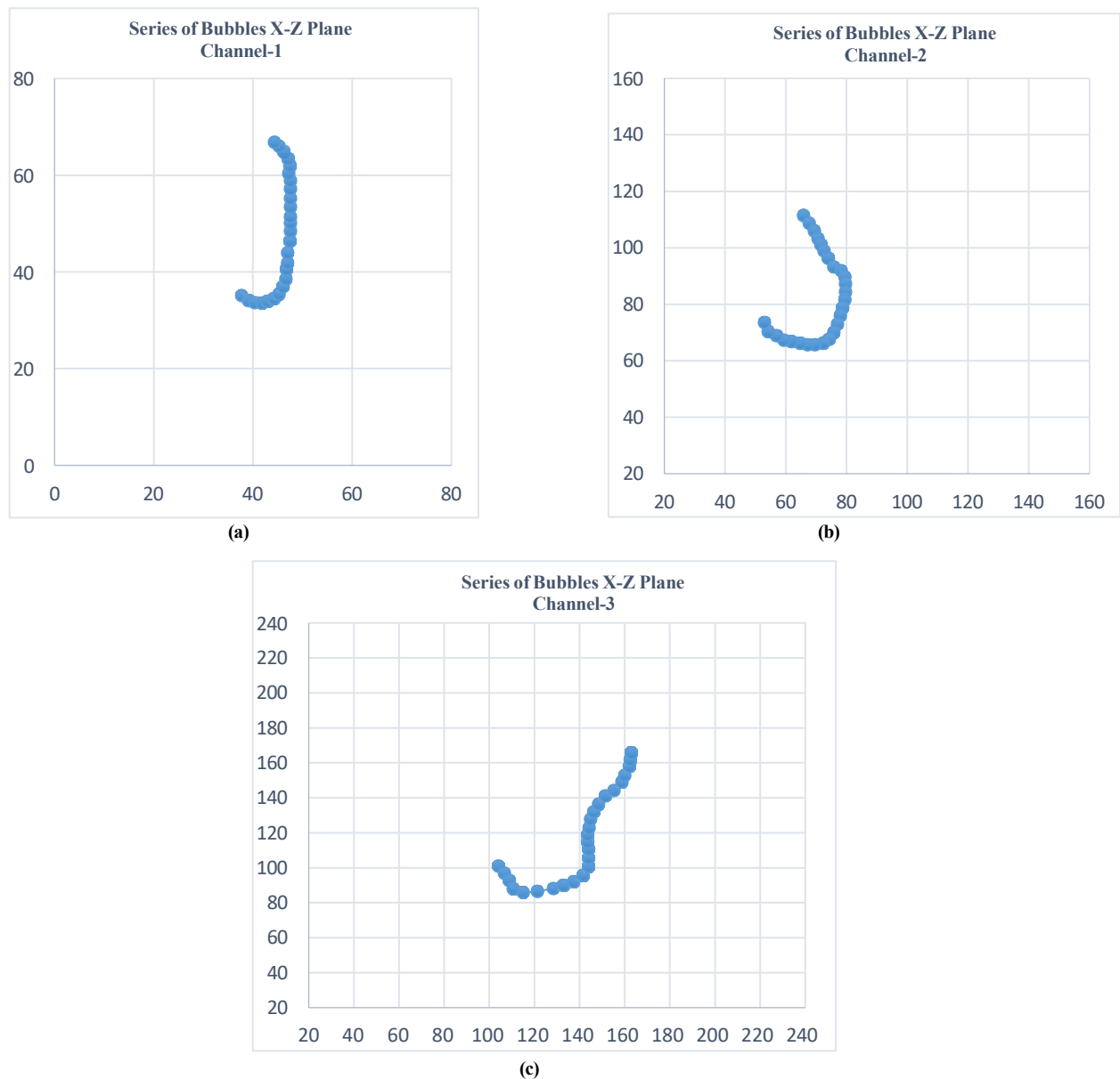
Figure 3.15(a-c): Graphical depiction of series of bubble's rise in x-z plane.
