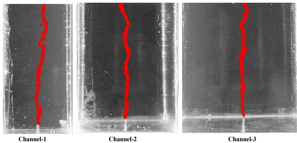
Figure 3.2: Trajectories of single bubble rise in water channels.
