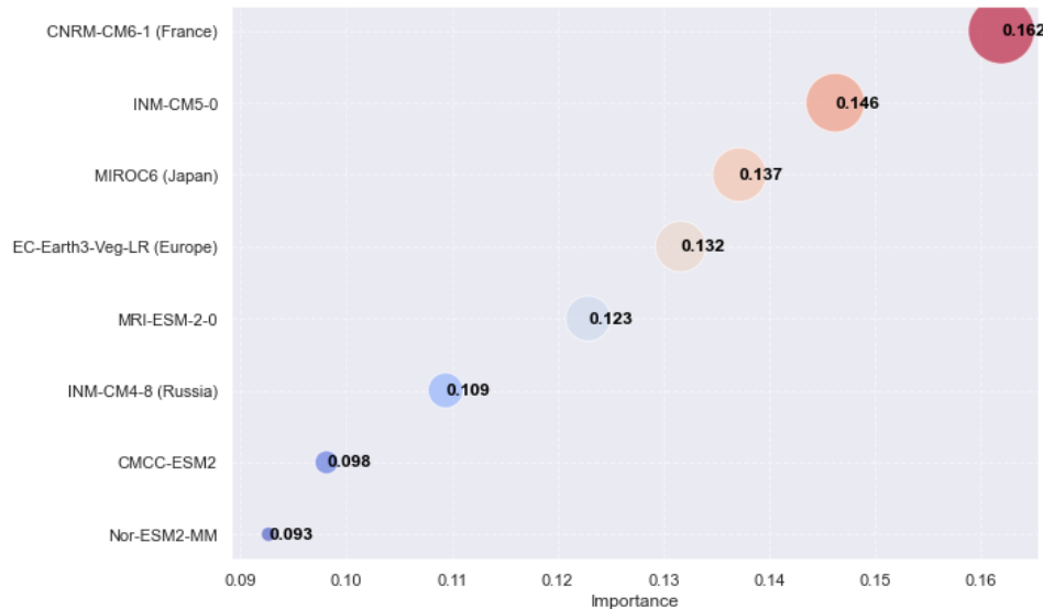
Figure 5 | GCM selection
